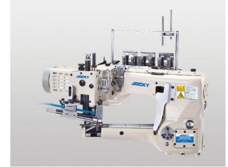
JK62GD-01 直驱曲臂式拼缝机 Direct drive 4-needle 6-thread feed-off-the-arm interlock sewing machine
