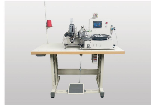
JK1377DD-XD988 自动送扣钉扣机 Automatic button attaching machine with auto button feeding device
