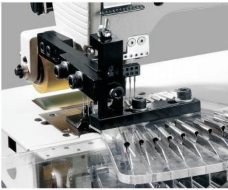
PSF: Shirt front attaching
