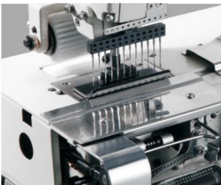
PTV: Shirt pleat / tuck fabric seaming
